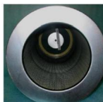
OR/R13 Size: 325 Dout=325mm, Din= 215mm, Hole in the bottom cap = 13 mm.
